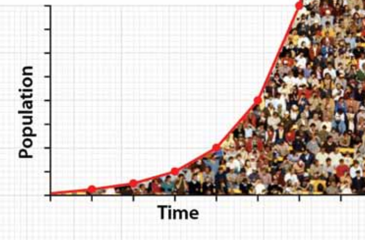
Exponential Communication
